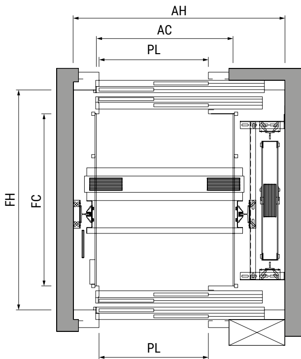
Plan view
